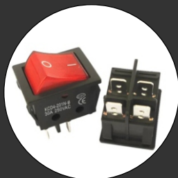
CHAVE GANGORRA ON-OFF 4 PINOS 30A
